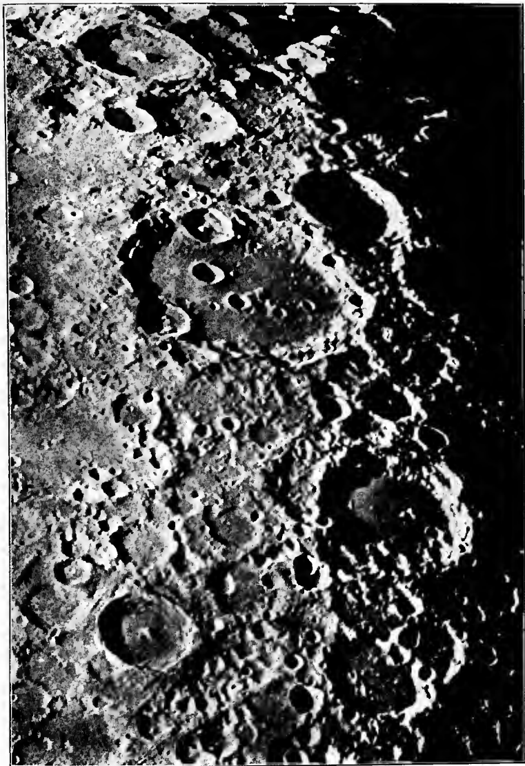
THE CRATERS CLAVIUS, LONGOMONTANUS, TYCHO, ETC.
